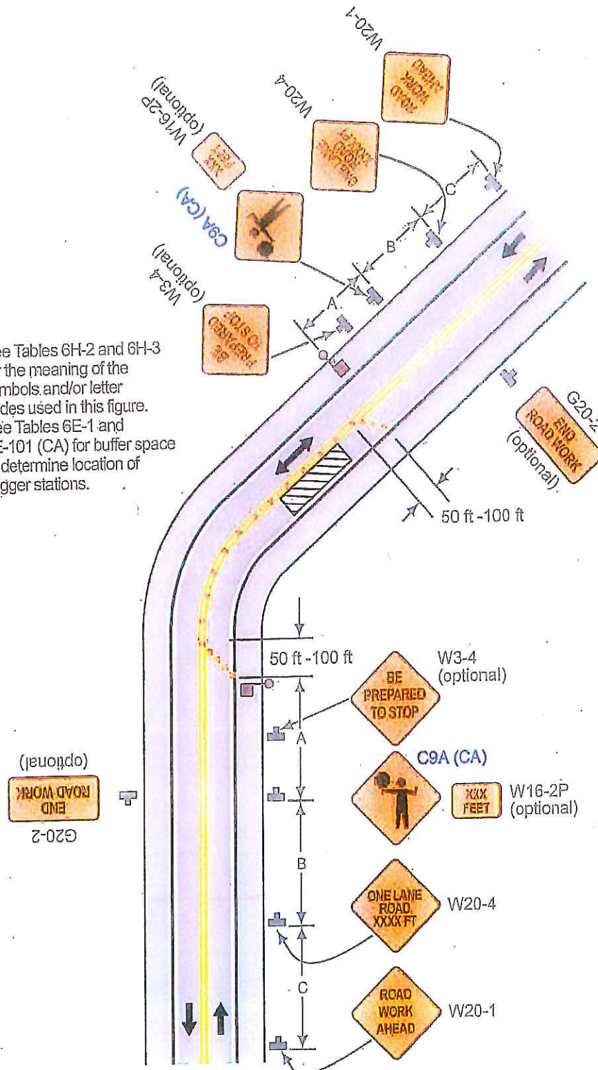
Typical Application 10
